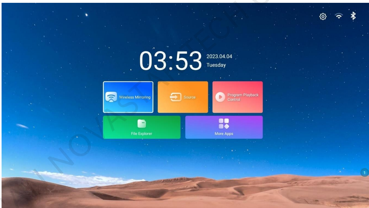
Figure 2-7 Home screen
